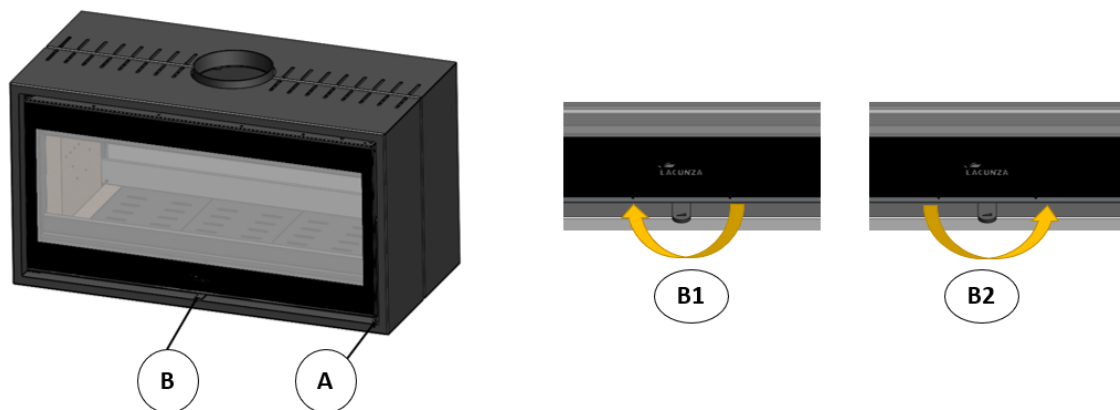
Figure No.17 - Operating components on the appliance
