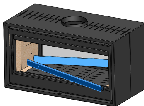
Figure No.18 - Removing the two separators.
