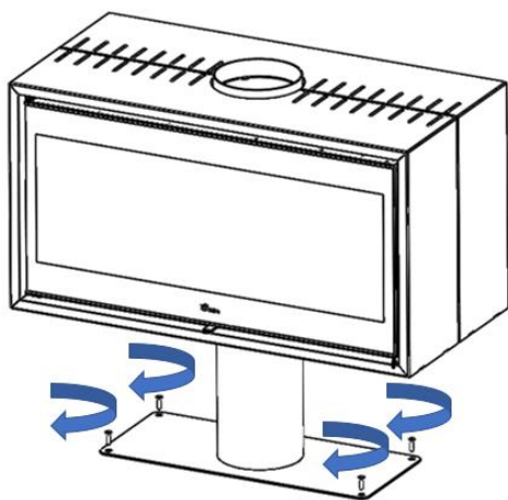
Figure No.7 - Fastening the Verona appliance to the floor
