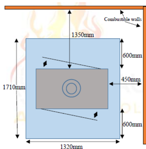
Figure No.9 - Safety distances for Verona 1000/1001/1003
