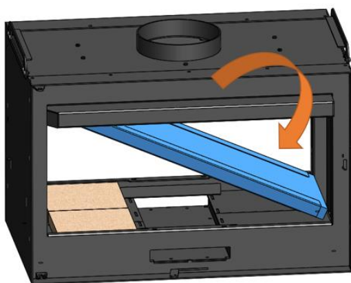
Figure No.22 - Drop the refractory holding it
