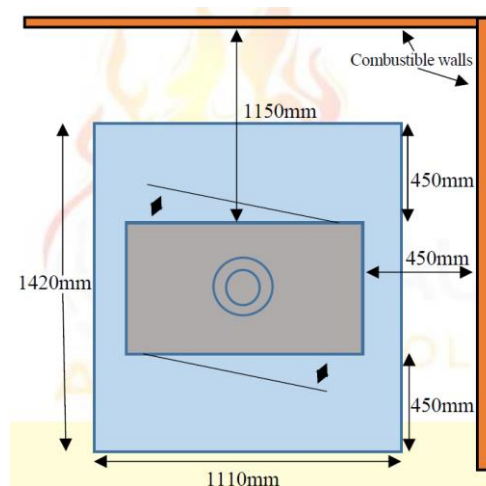
Figure No.8 - Safety distances for Verona 800/801
