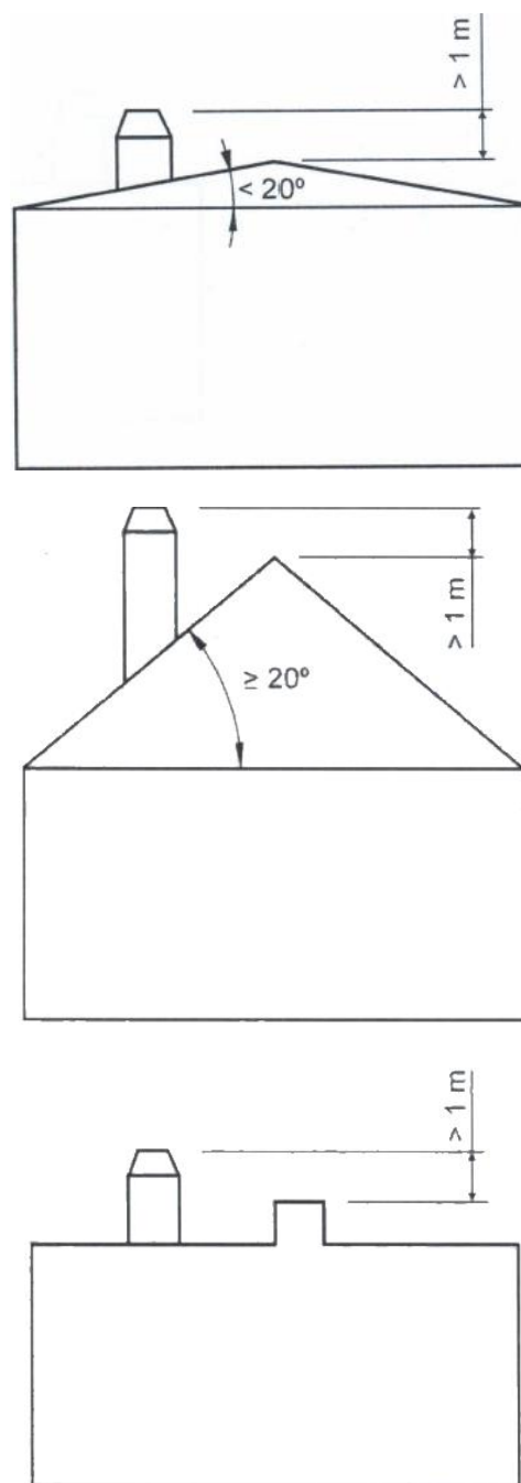
Figure No.13 - Distances between chimney crown and roof ridge
