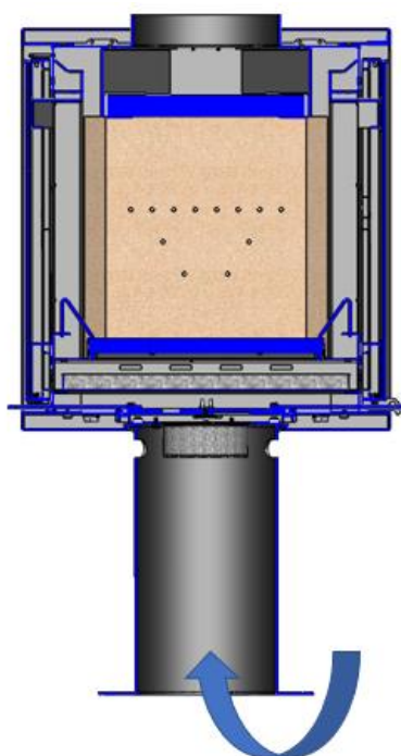
Figure No.11 - Piping air to the firebox in Verona 1001
