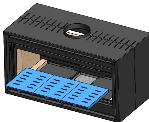
Figure No.19 - Removing the cast iron grilles
