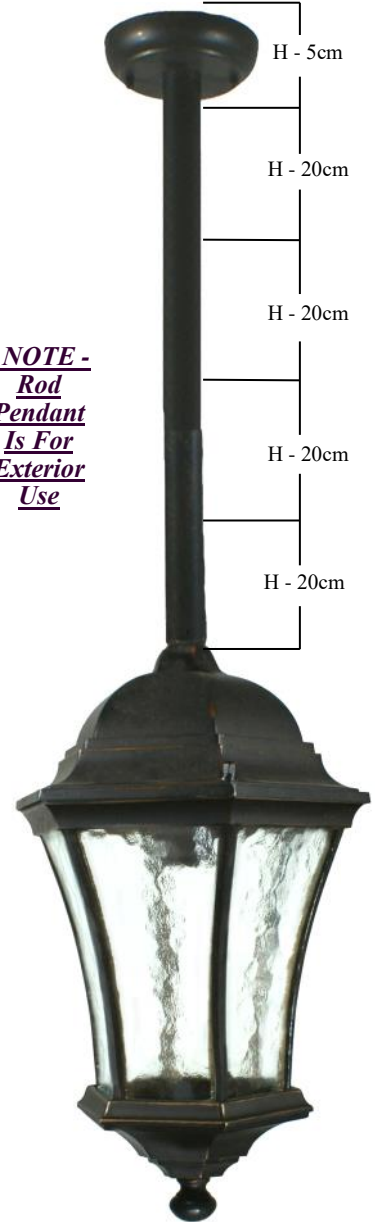
1000491 STRAND MEDIUM ROD PND E27 FRAME SIZE H - 39cm W - 24cm + 4 x 20cm RODS + 1 x 5cm CAP
