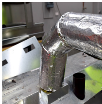
Flue Discharge Connection
