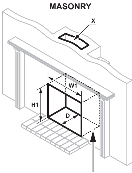
Level base with a slurry of sand and cement.
